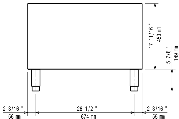
Lateral
