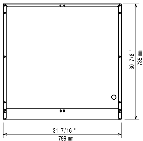
Lateral
