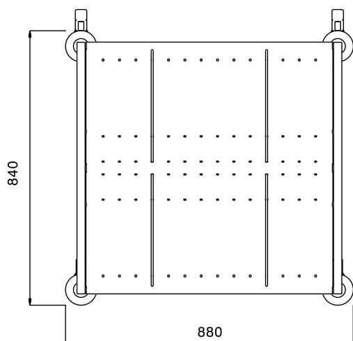
Lateral
